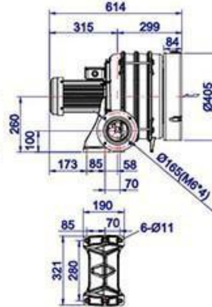
HTB100-304 4-stage
