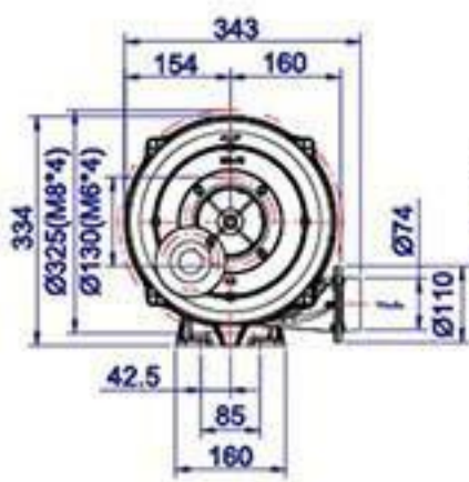
HTB75-105 5-stage
