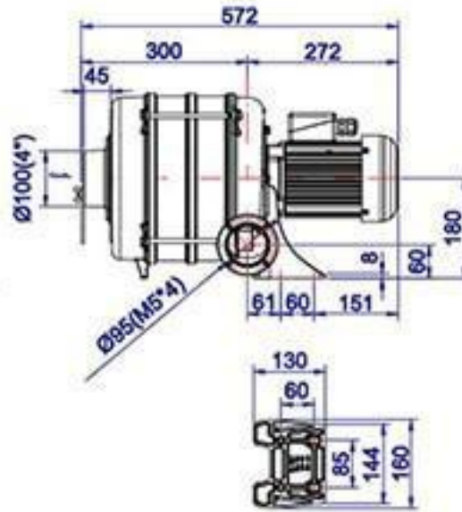
HTB75-104 4-stage
