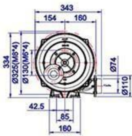
HTB75-053 3-stage
