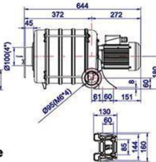
HTB75-105 5-stage
