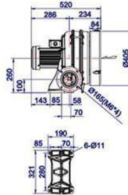
HTB100-203 3-stage
