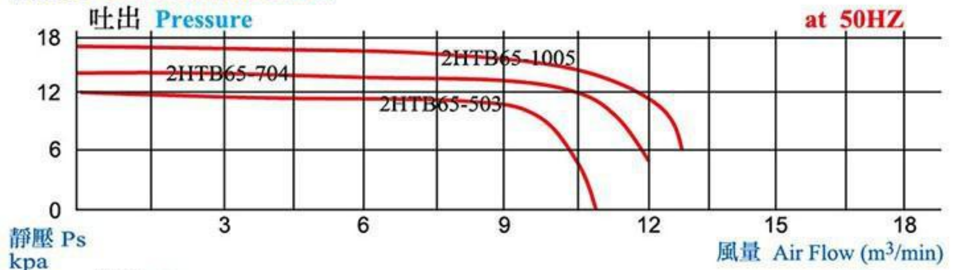
性能表 Characteristic curves
