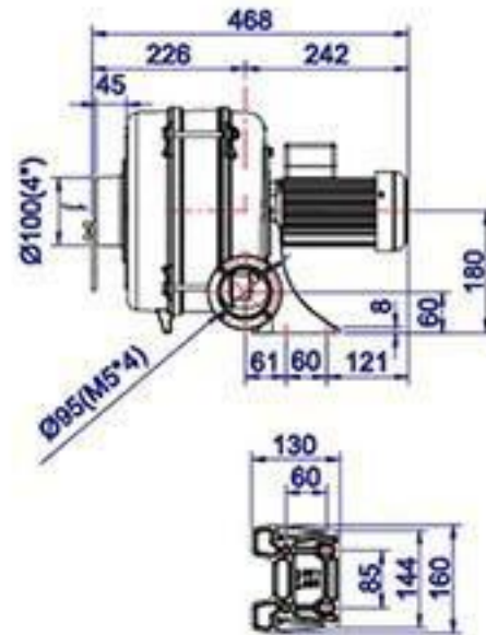
HTB75-053 3-stage
