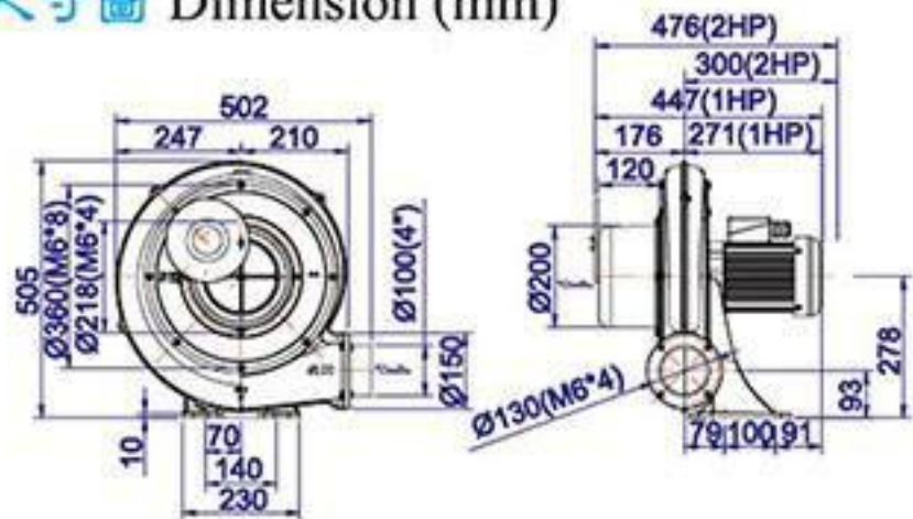
TB100-1 / TB100-2
