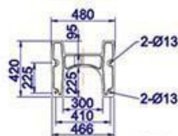
TB200-15 / TB200-20
