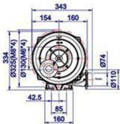
HTB75-104 4-stage
